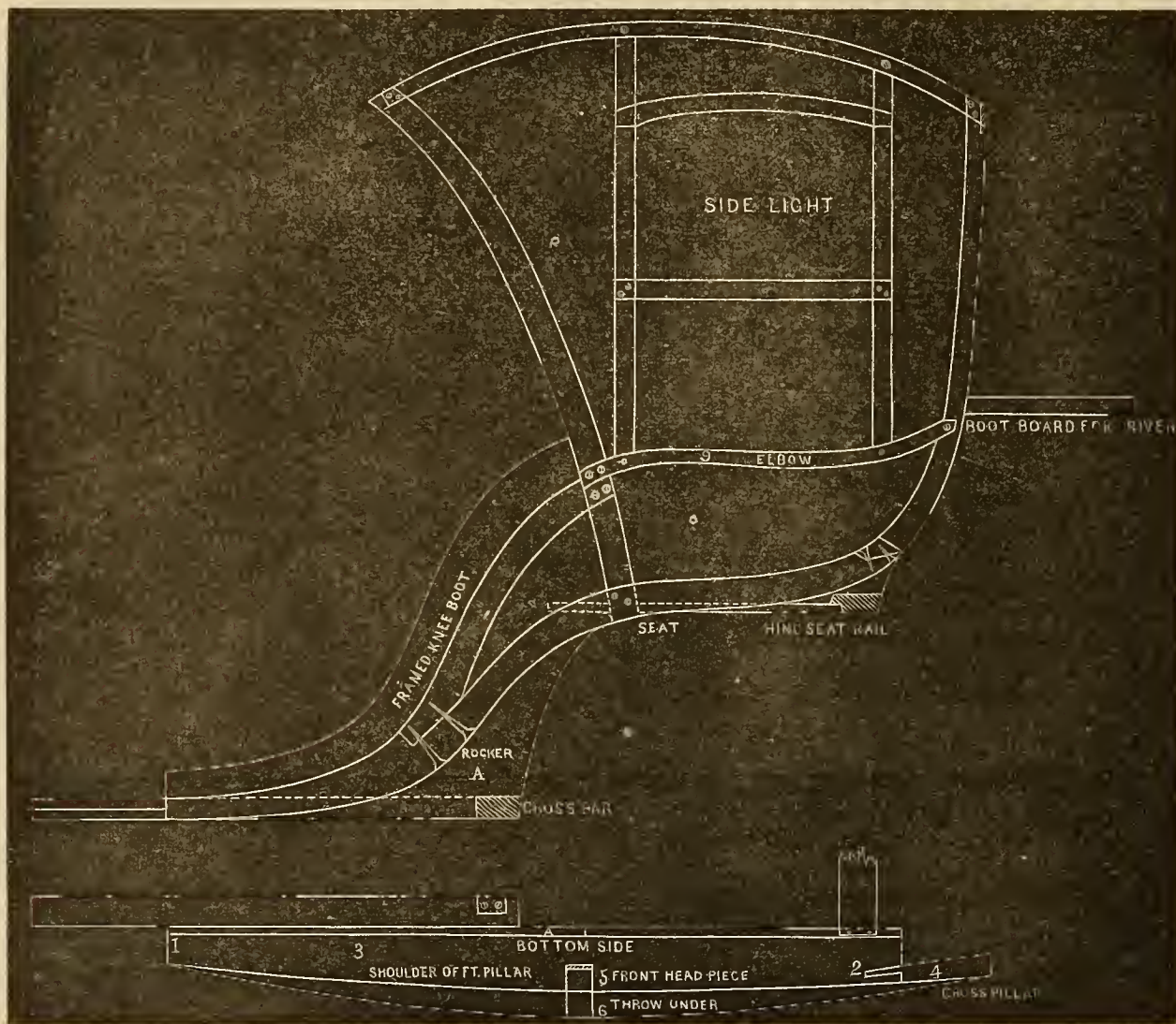
PRIVATE HANSON, WITH CANT-BOARD.— \frac{1}{2} IN. SCALE.
